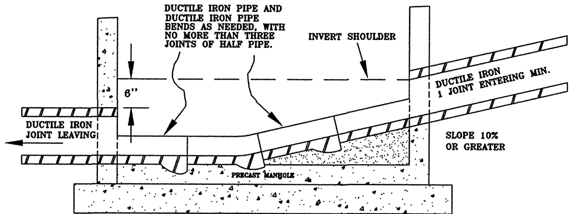
SECTION ALONG CENTER LINE OF PIPE
