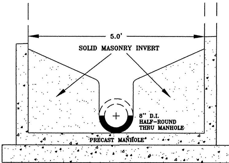
SECTION AT RIGHT ANGLE TO CENTER LINE OF PIPE
