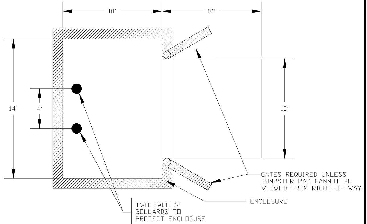
PLAN VIEW
