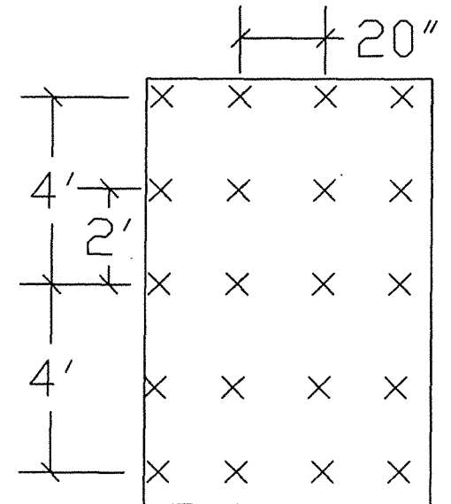
TYPICAL STAPLE PATTERN "D"
