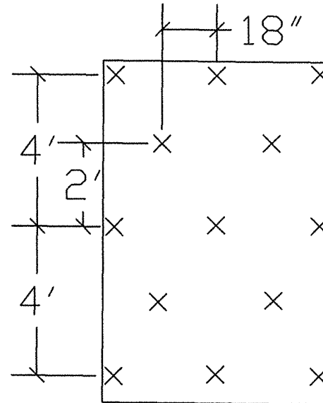
TYPICAL STAPLE PATTERN "C"
