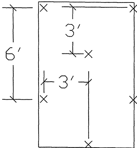
TYPICAL STAPLES #8 GAUGE WIRE
