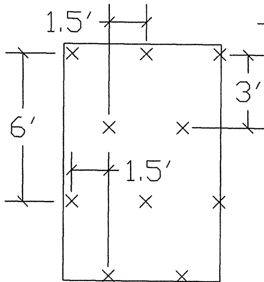
TYPICAL STAPLE PATTERN "B"
